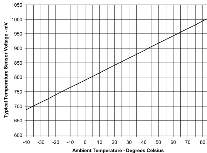
Figure 10. Typical Temperature Sensor Voltage
